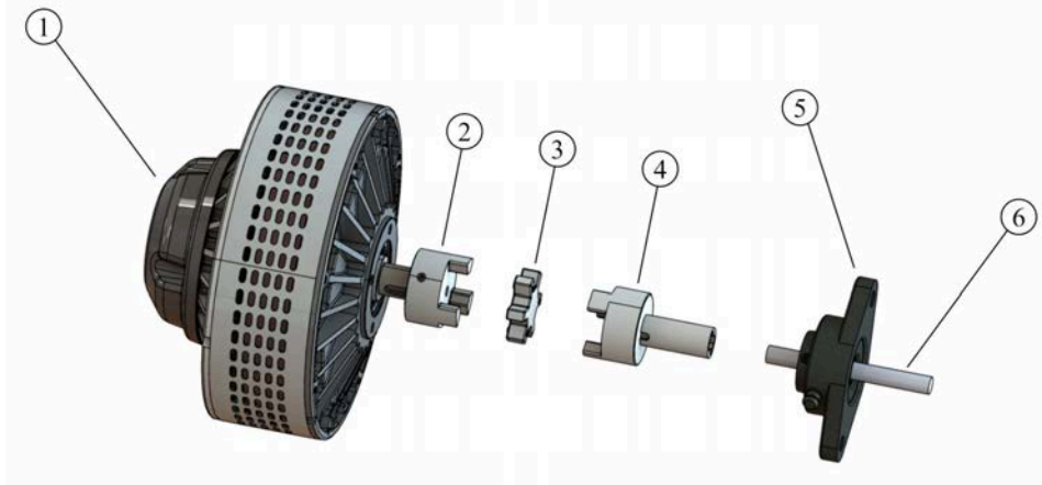
Figure 10: An exploded view of the main drivetrain components in the upper unit; left to right: ① Motor, ② Upper jaw coupling, ③ Rubber “spider”, ④ Lower jaw coupling and shaft adapter, ⑤ Bearing, ⑥ Outboard shaft
