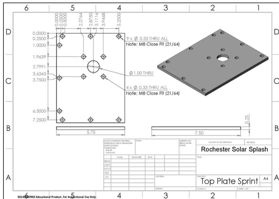
The upper plate is used for the sprint motor. Similarly, the sprint motor is permanently attached to this plate, and the plate is used to switch out motors.
