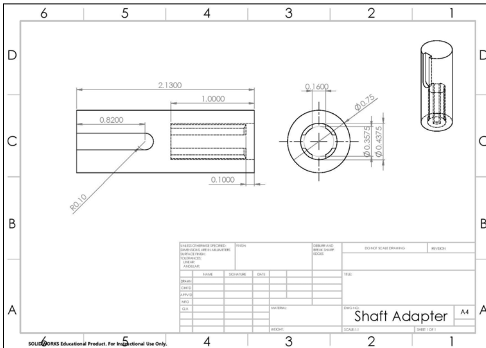
A shaft adapter is used to connect the upper unit to the 4-spline outboard motor shaft.
