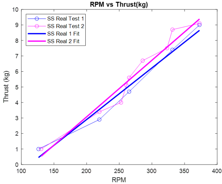
RPM vs. Thrust results for two different testing sessions on the real Solar Splash propeller.
