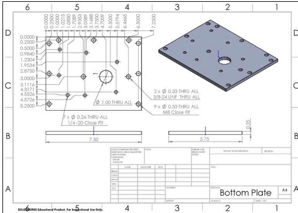
The drivetrain bottom plate bolts to the outboard motor unit.
