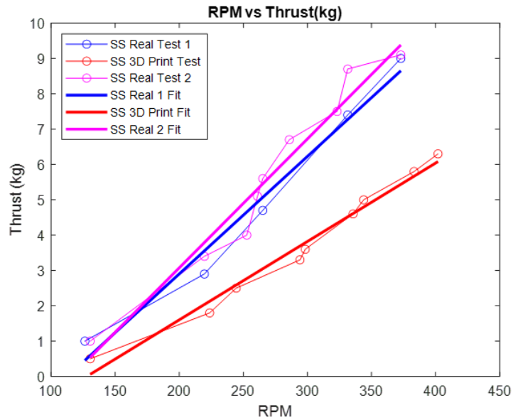
Compare SS 3D printed to SS actual testing.
