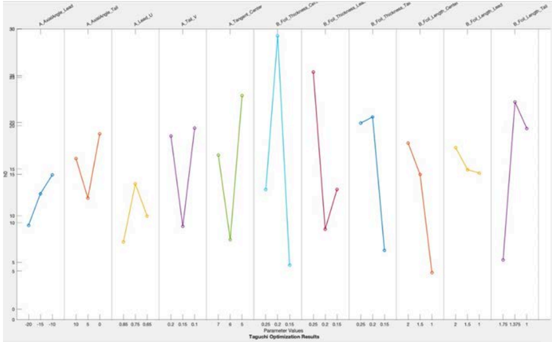
Round two results of Taguchi Method optimization examining eleven parameters with three levels of values.
