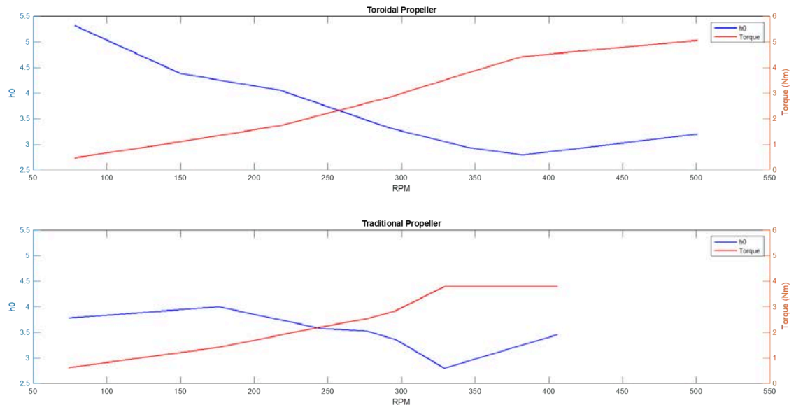
Figure 15: Efficiency toroidal compared to current, traditional propeller based on the RPM.
