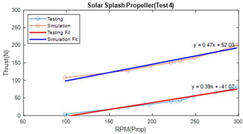
Correlating SS Simulation to SS testing data.
