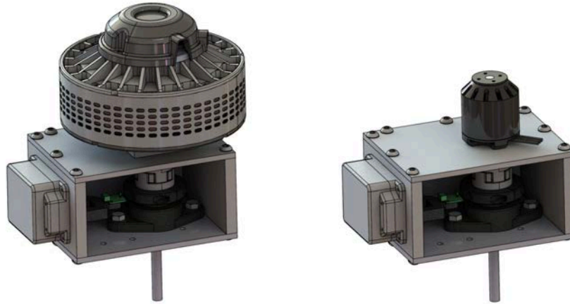
Figure 9: Left: The upper drive unit is shown with the sprint motor installed. Right: The upper drive unit is shown with the endurance motor installed. Note the bolts on the upper plates, which are unscrewed to change which motor is used in the assembly.
