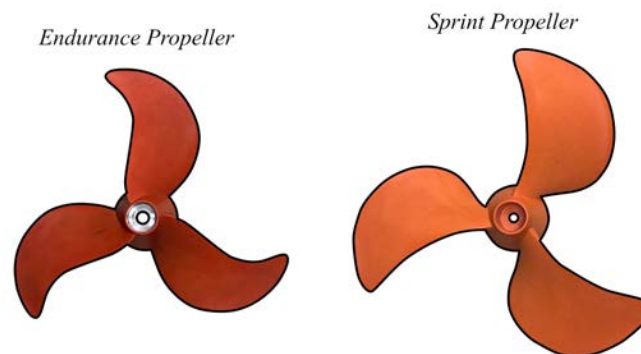
Figure 13: Left: The Torqeedo v8/p350 propeller is used for endurance competitions.
