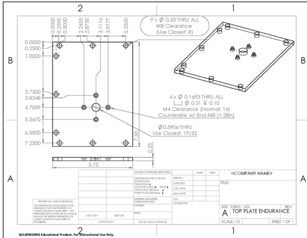
The upper plate used for the endurance motor. The endurance motor is permanently attached to this plate, and the plate is used to switch out motors.
