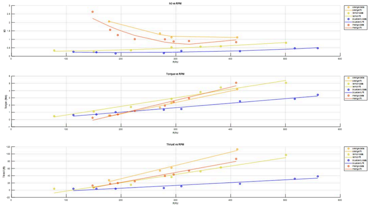
Comparing all the different propellers against each other.
