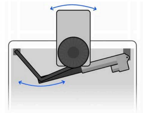
Figure 16: Linear Actuator Movement.
